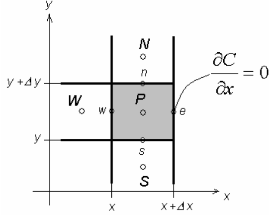
Fig. 4. Boundary control volume with zero derivative boundary condition
